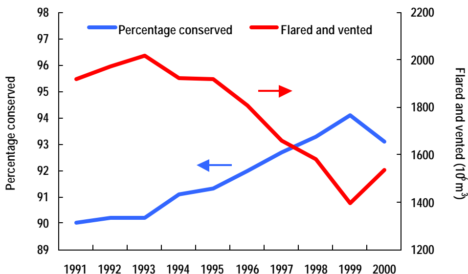
Figure 1. Percentage of solution gas conserved
