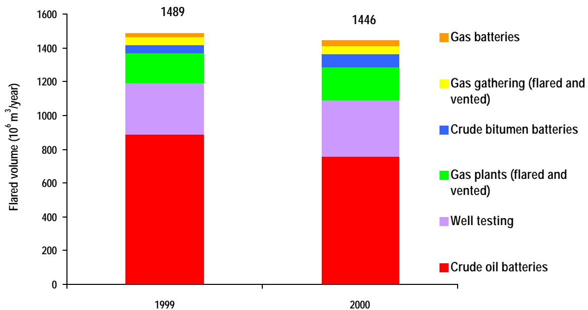
Figure 3. Flaring from upstream oil and gas sources
