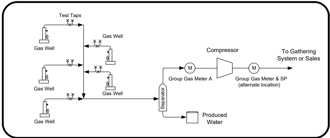
Figure 8.1 Shallow gas or coalbed methane wells
