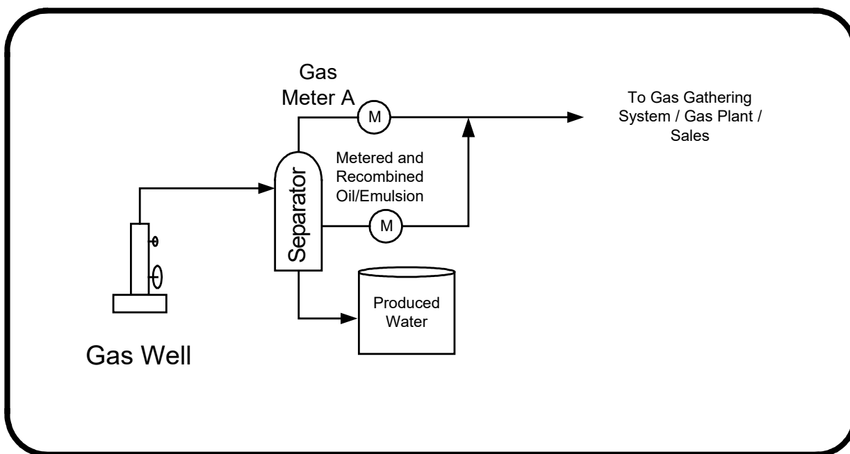
Figure 8.7 Oil production
