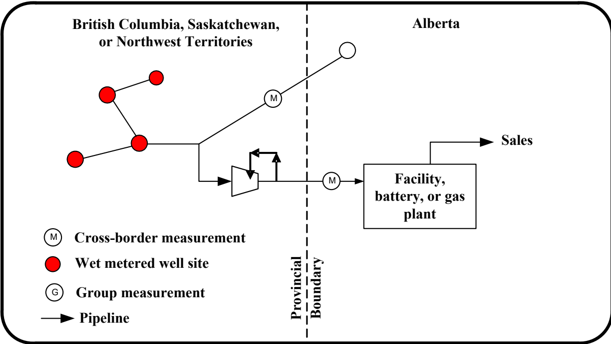
Figure 9.3 Multiple jurisdictional crossing
