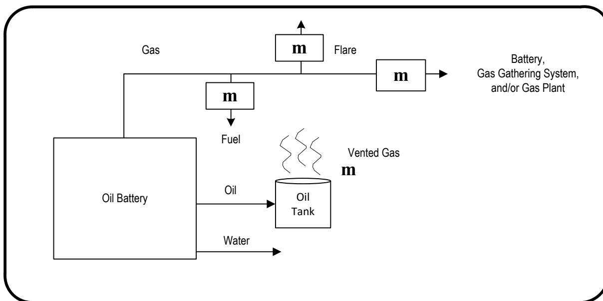
Figure 1.2 Total battery gas
