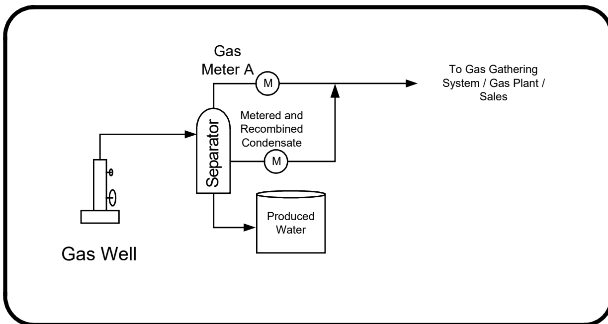
Figure 8.6 Condensate production
