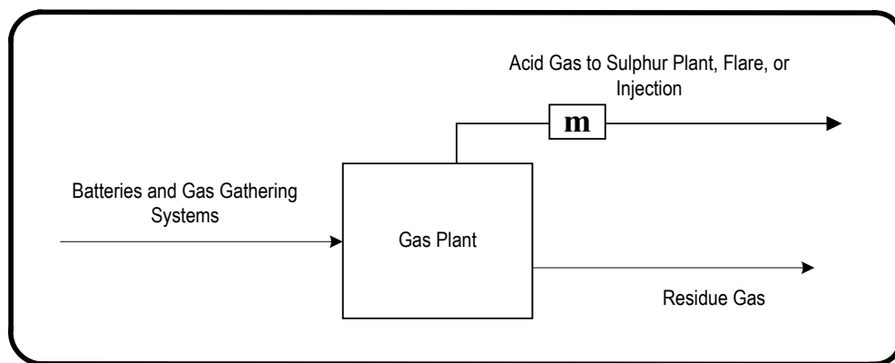
Figure 1.13 Acid gas
