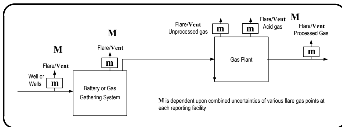
Figure 1.12 Flare and vent gas
