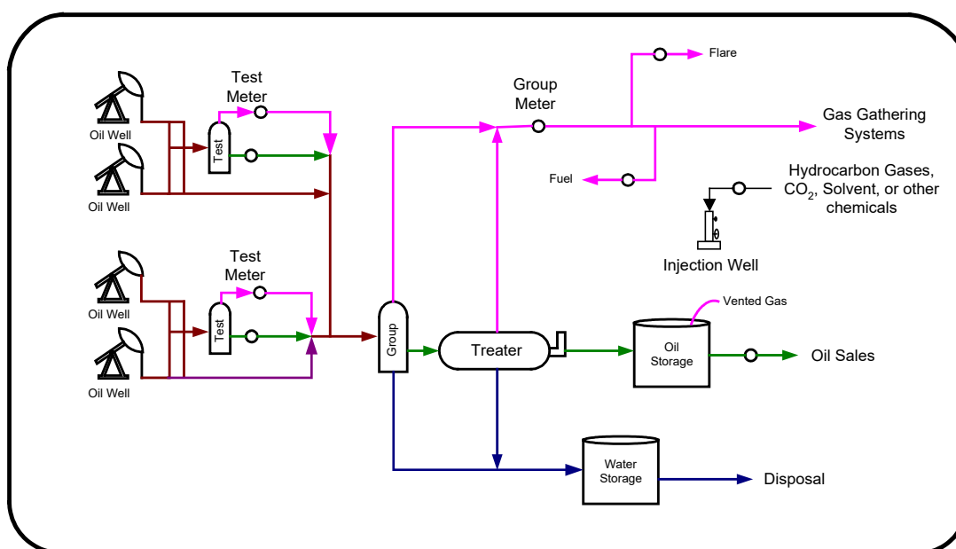
Figure 8.14 Miscible/immiscible flood
