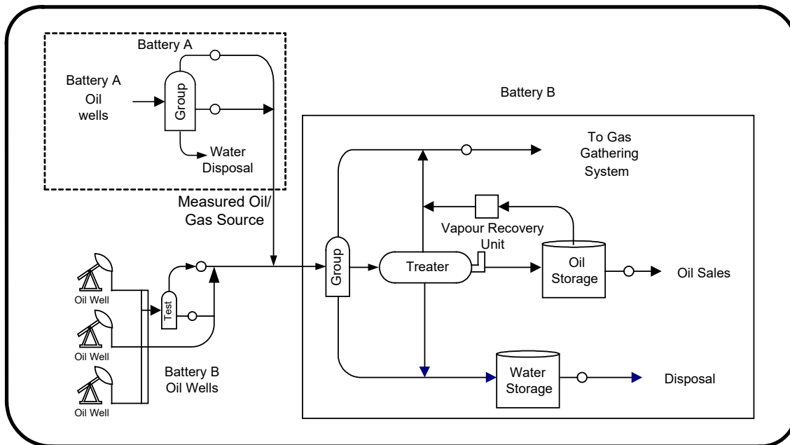
Figure 5.11 Measured oil or oil emulsion (and gas if applicable) under pressure from a battery delivering into a crude oil multiwell proration battery by pipeline
