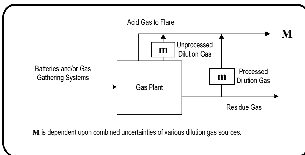
Figure 1.14 Dilution gas
