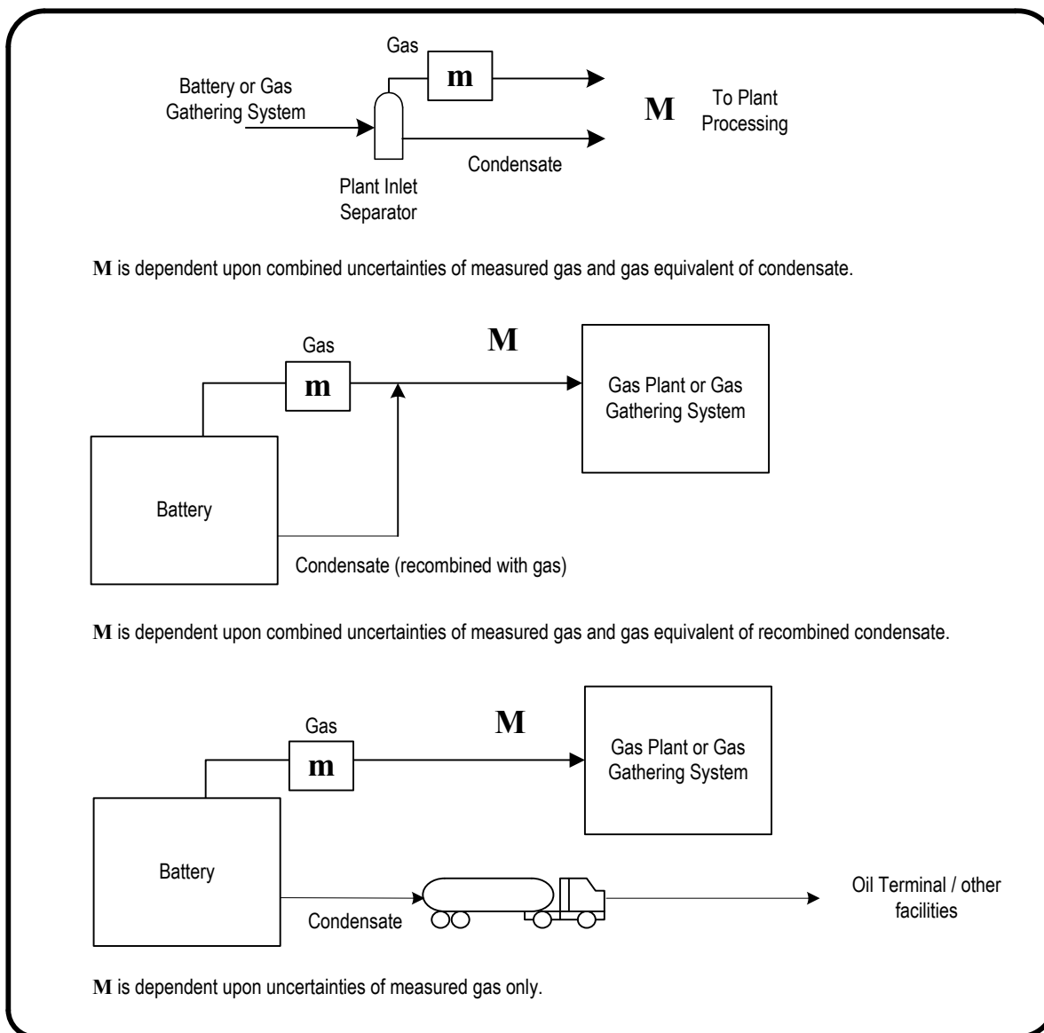
Figure 1.9 Plant inlet or total battery/group gas
