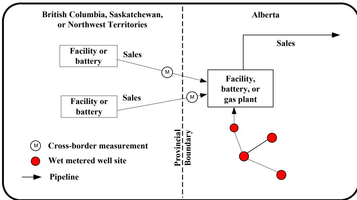
Figure 9.5 Sales gas source from an out-of-province location
