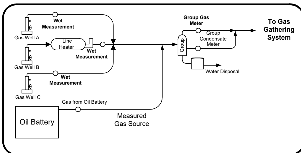
Figure 5.6 Measured oil facility gas delivering into a gas proration battery
