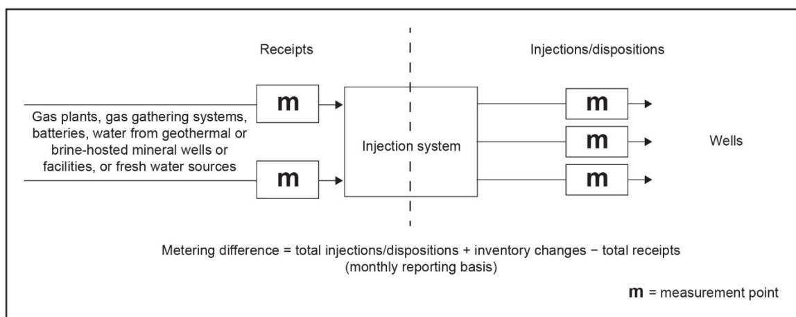
Figure 3.3 Injection/disposal systems
