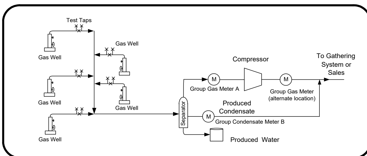
Figure 8.2 Gas multiwell proration outside SE Alberta battery
