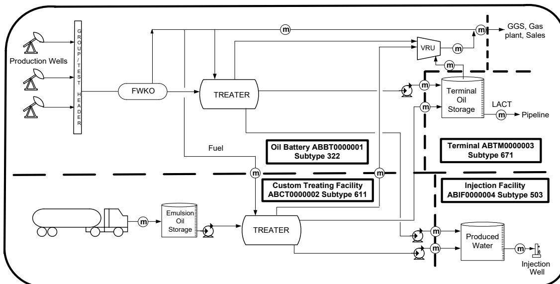
Figure 10.3 Custom treating, oil battery, and terminal schematic – scenario 2
