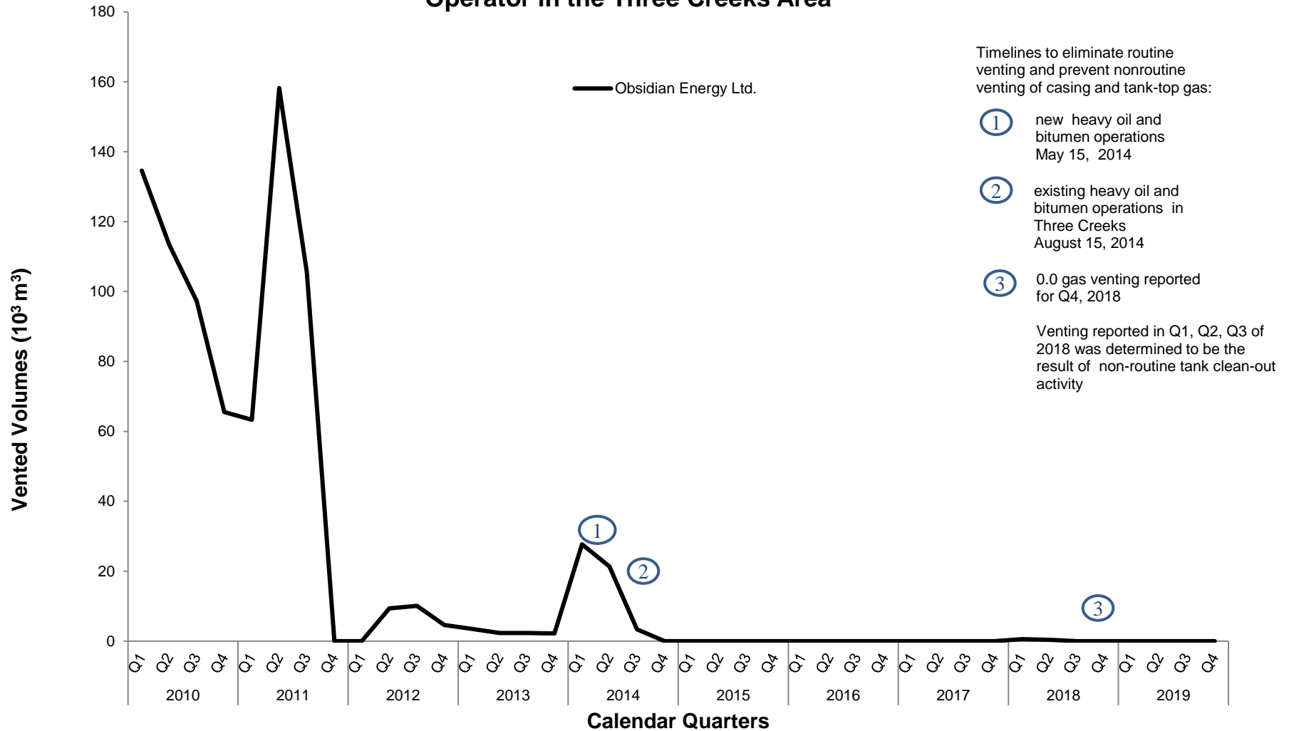
Figure 7 – Vented Gas Reported to Petrinex from Oil and Bitumen Batteries by Each Operator in the Three Creeks Area
