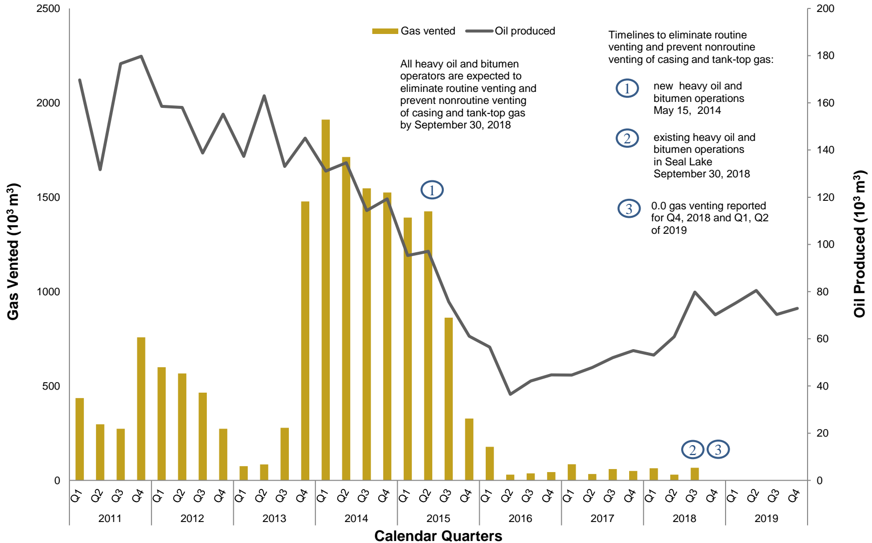
Figure 5 – Vented Gas and Oil Production Reported to Petrinex from Oil and Bitumen Batteries in the Seal Lake Area
