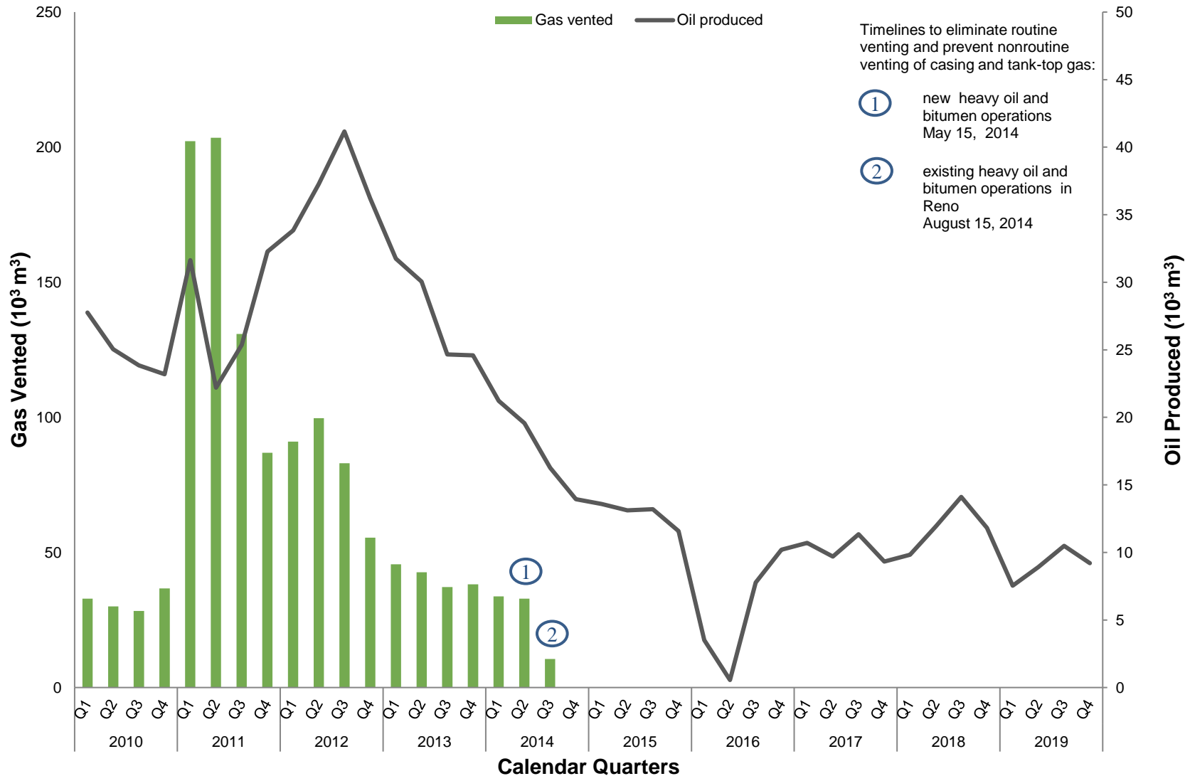
Figure 4 – Vented Gas and Oil Production Reported to Petrinex from Oil and Bitumen Batteries in the Reno Area
